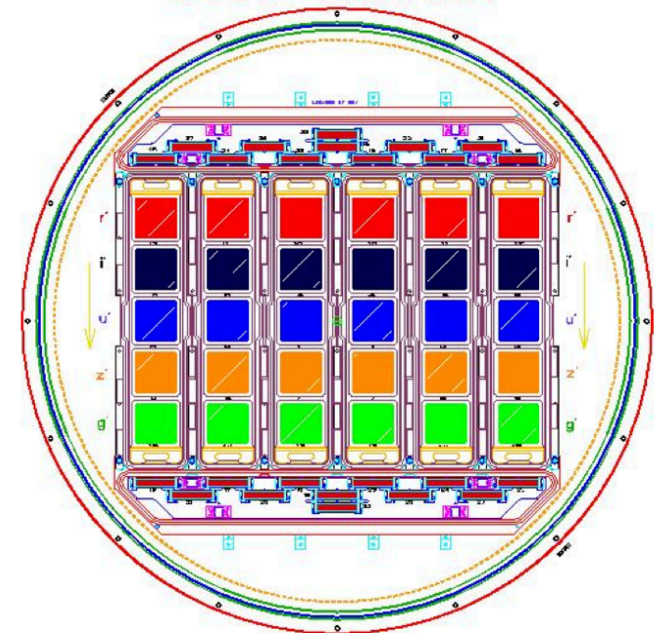
SDSS CAMERA
